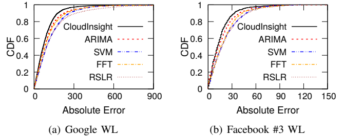
Fig. 6. CDF of prediction errors in two cluster workloads
