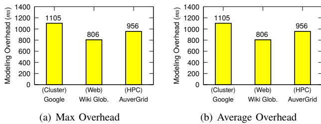
Fig. 9. Modeling overhead of CloudInsight
